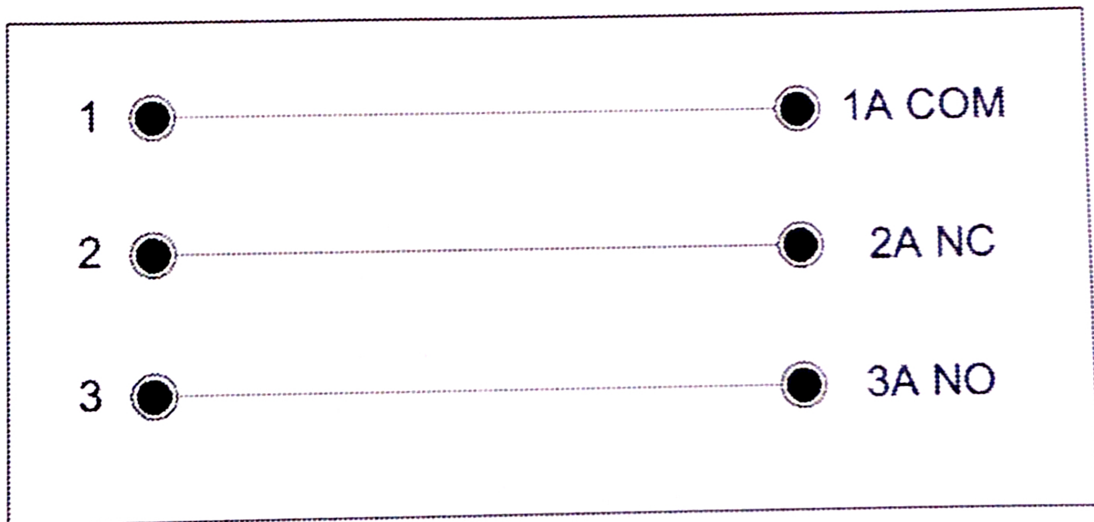
WS900 Connection Diagram To Conventional Fire Panel
